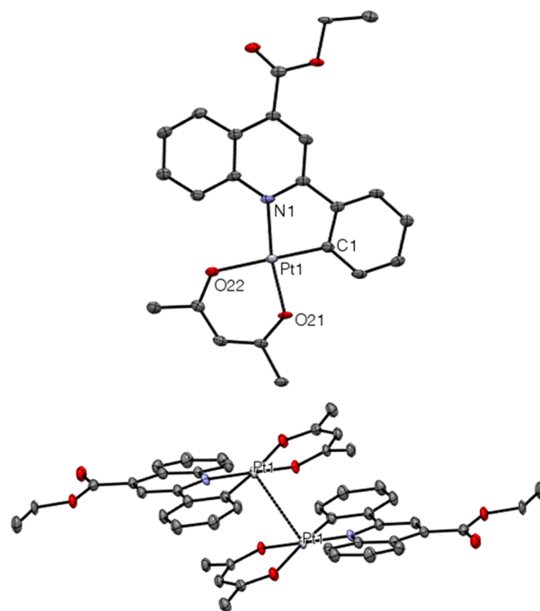
Figure 1. X-ray crystal structure of [Pt(L1)(acac)] (top) and the Pt–Pt interaction (bottom). Hydrogen atoms omitted for clarity. The ellipsoid probabilities are at 50%.
