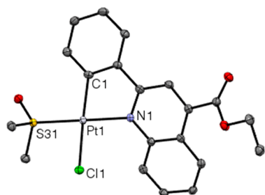
Figure 2. X-ray crystal structure of [\text{PtCl}(\text{L1})(\text{DMSO})] . Hydrogen atoms omitted for clarity. The ellipsoid probabilities are at 50%.
