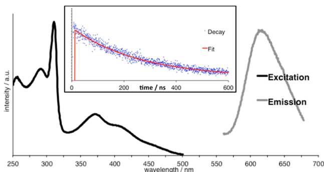
Figure 6. Excitation ( \lambda_{\text{em}} = 615 nm) and emission ( \lambda_{\text{ex}} = 425 nm) spectra for [\text{Pt}(\text{L1})(\text{hfacac})] ( \lambda_{\text{ex}} = 425 nm). (inset) Fitted ( \tau = 262 ns) monoexponential decay profile for [\text{Pt}(\text{L1})(\text{hfacac})] ( \lambda_{\text{ex}} = 372 nm).
