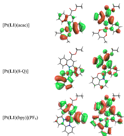
Figure 4. Calculated representations of HOMO (left) and LUMO (right) for selected complexes.
