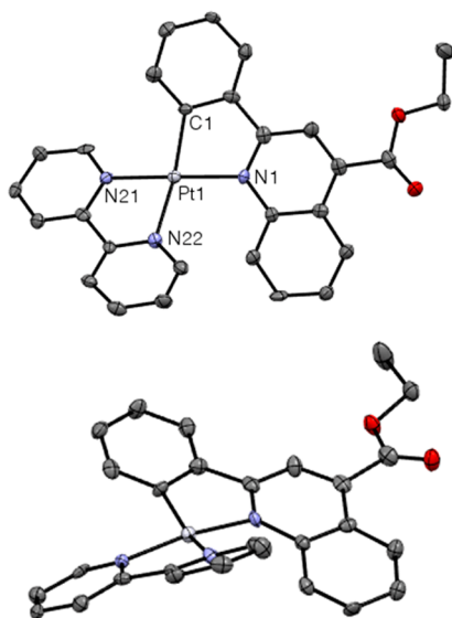
Figure 3. X-ray crystal structure of [\text{Pt}(\text{L1})(\text{bpy})](\text{PF}_6) . Hydrogen atoms and \text{PF}_6^- counteranion omitted for clarity. The ellipsoid probabilities are at 50%.
