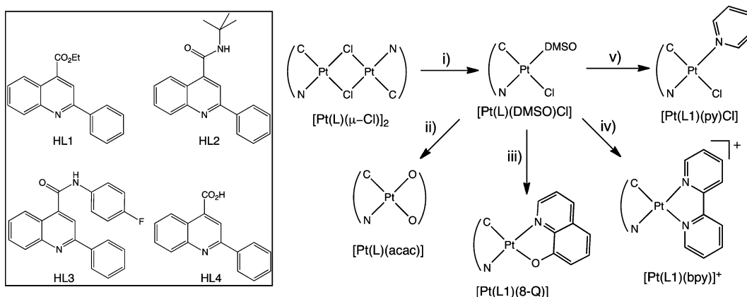
Scheme 1. Ligands (Inset) and the Reaction Pathways to the Various Cyclometalated Pt(II) Complexes a
