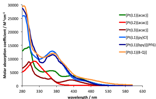
Figure 5. UV-vis absorption profiles for selected complexes in solution (all measured in CHCl 3 except [Pt(L1)(bpy)](PF 6 ) in MeCN).
